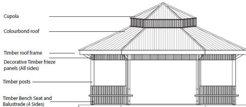
A ELEVATION SCALE 1:50
